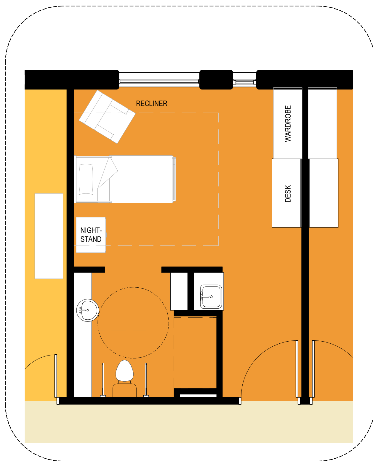
MEMBER UNIT - TYPICAL 1/4" = 1'-0"
